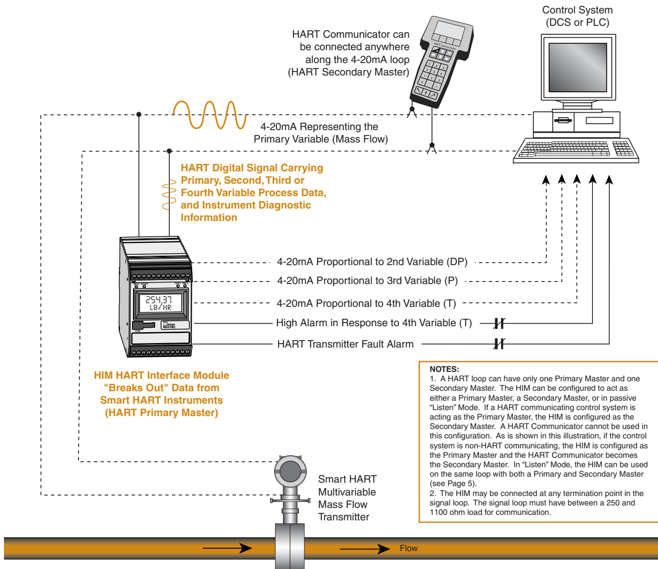
Figure 1. The HIM converts HART digital data to 4-20mA values proportional to a multi variable transmitter's primary, second, third or fourth variables. Its alarm trip outputs warn of unwanted high/low process conditions or of instrument diagnostic problems.
