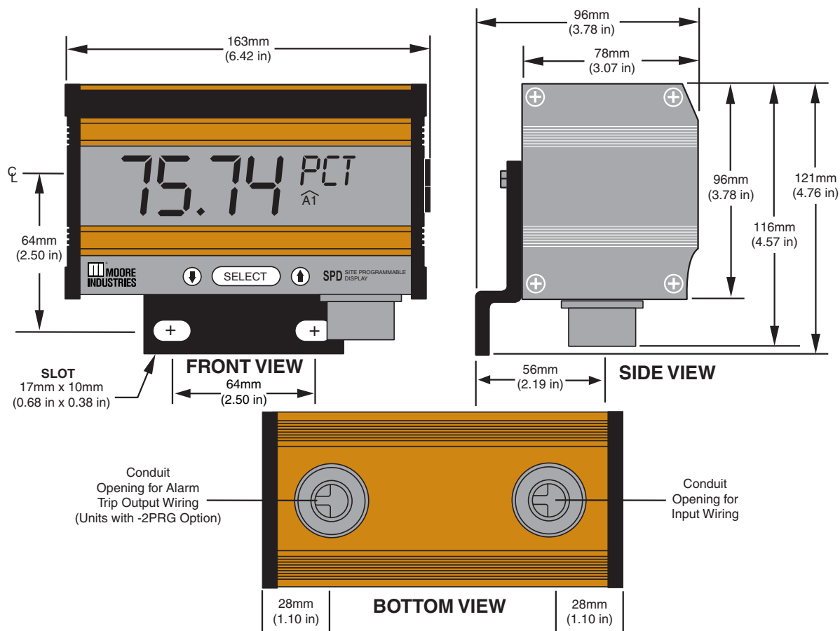
Figure 2. Installation Dimensions
